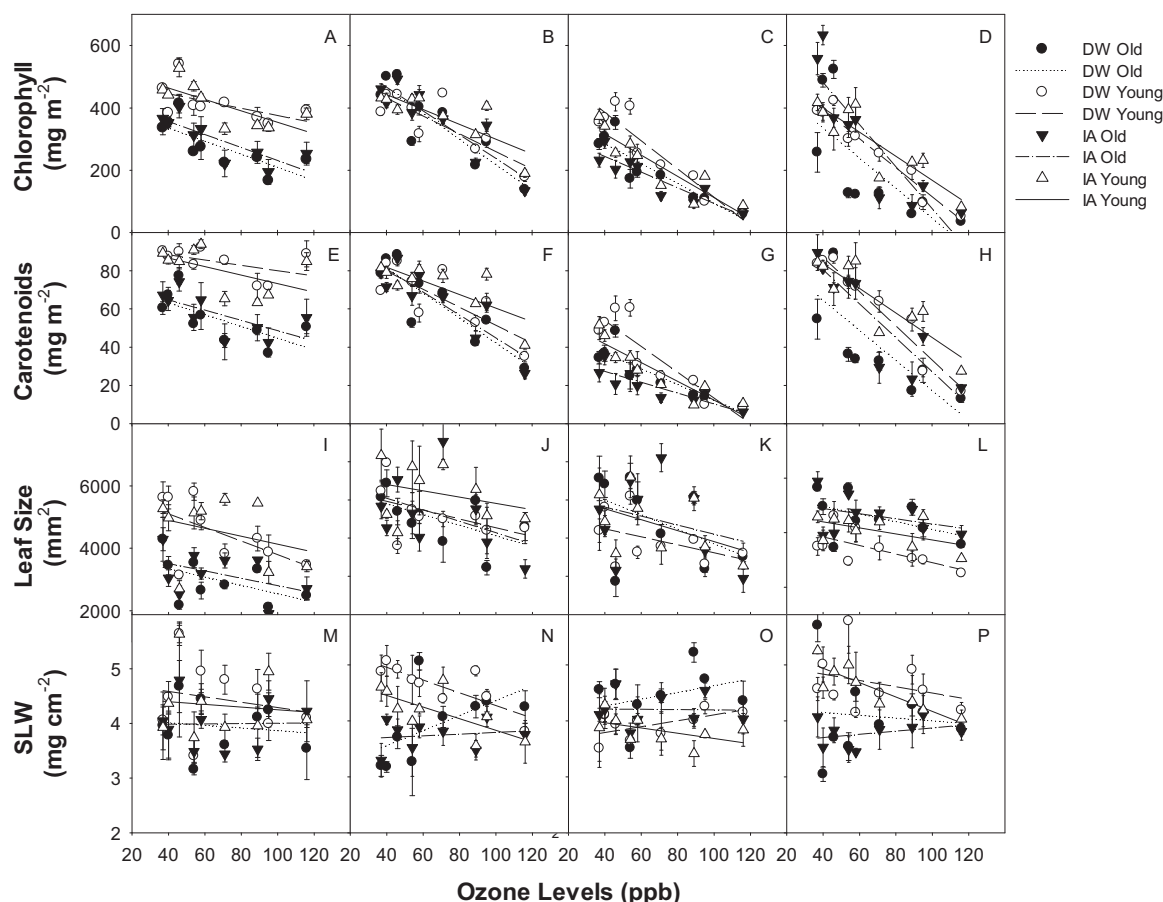
Fig. 2. Leaf total chlorophyll (Chl, A–D), carotenoids ( C_x , E–H), leaf size (I–L) and specific leaf weight (SLW, M–P) for the young leaves (open symbol) and old leaves (closed symbol) of the 2 cultivars (DW, circle; IA, triangle) under various ozone levels and developmental stages – R1 (A, E, I and M), R2 (B, F, J and N), R4 (C, G, K and O) and R5 (D, H, L and P). Linear regressions were fit for DW old (dotted line), DW young (dashed line), IA old (dot dash line) and IA young leaves (solid line), respectively. The overall relationships of Chl, C_x and leaf size with mean [O_3] (x) can be described as y = -3.38x + 526.0 , y = -0.506x + 89.2 , and y = -13.534x + 5672.5 , respectively. The overall R^2 values of Chl, C_x and leaf size with mean [O_3] were significant ( p < 0.0001 ).
