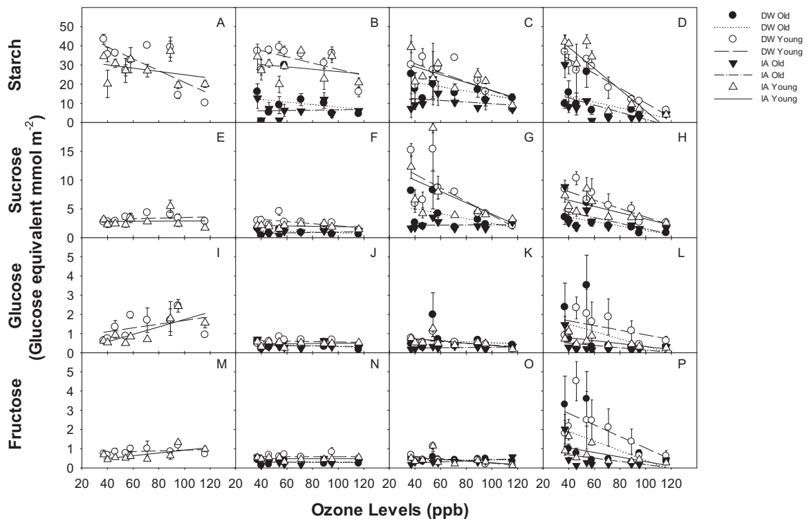
Fig. 8. Leaf starch (A–D), sucrose (E–H), glucose (I–L) and fructose (M–P) analyzed with enzymatic method for the young leaves (open symbol) and old leaves (closed symbol) of the 2 cultivars (DW, circle; IA, triangle) under various ozone levels and developmental stages – R1 (A, E, I and M), R2 (B, F, J and N), R4 (C, G, K and O) and R5 (D, H, L and P). Linear regressions were fit for DW old (dotted line), DW young (dashed line), IA old (dot dash line) and IA young leaves (solid line), respectively. The overall relationships of starch and sucrose with mean [O_3] ( x ) can be described as y = -0.199x + 33.82 and y = -0.031x + 5.582 , respectively. The overall R^2 values of starch and sucrose with mean [O_3] were significant ( p < 0.0001 ).
