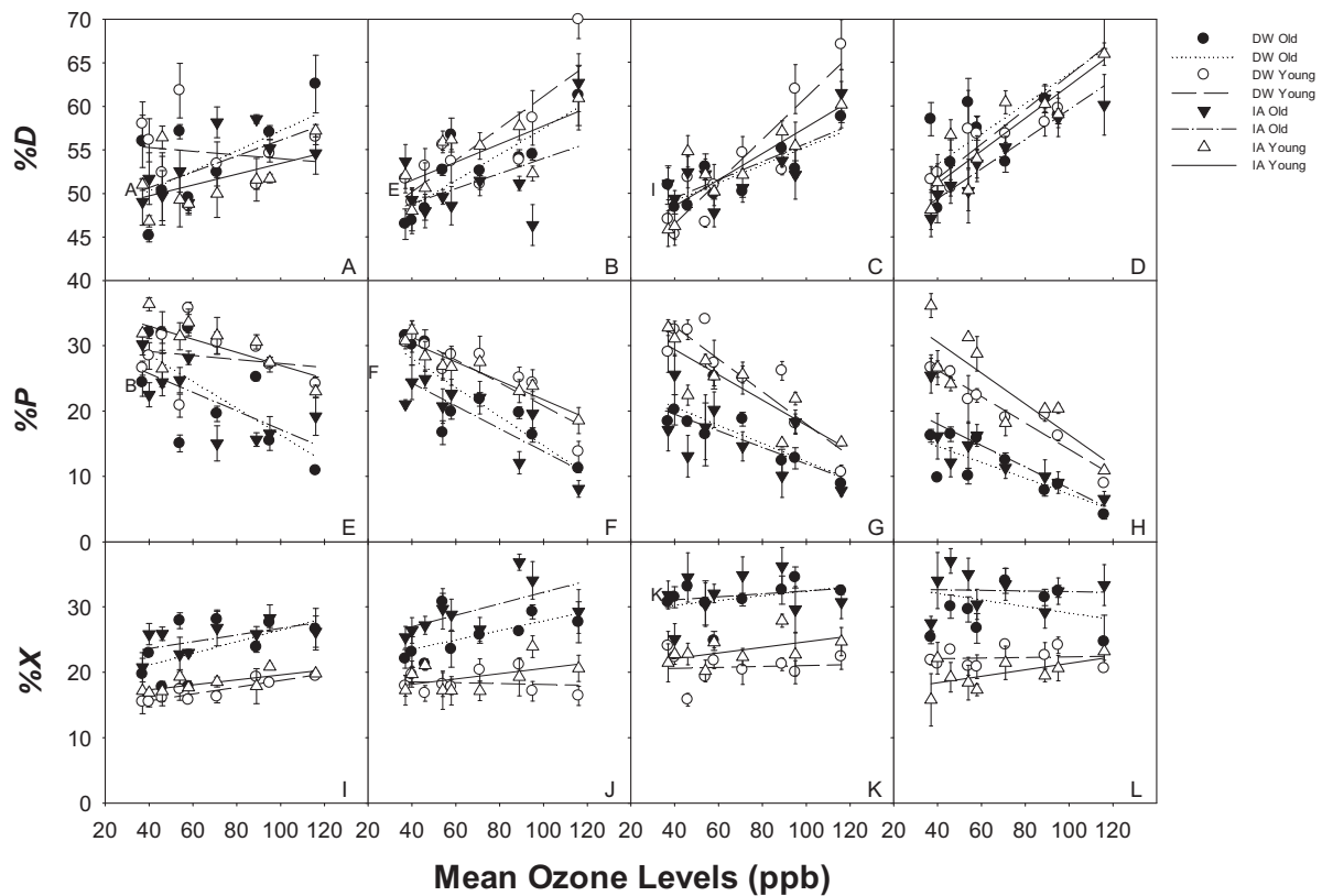
Fig. 7. %D (A–D), %P (E–H) and %X (I–L) for the young leaves (open symbol) and old leaves (closed symbol) of the 2 cultivars (DW, circle; IA, triangle) under various ozone levels and developmental stages – R1 (A, E and I), R2 (B, F and J), R4 (C, G and K) and R5 (D, H and L). Linear regressions were fit for DW old (dotted line), DW young (dashed line), IA old (dot dash line) and IA young leaves (solid line), respectively. The overall relationships of %D, %P and %X with mean [O_3] ( x ) can be described as y = 0.13x + 44.8 , y = -0.1626x + 32.9 , and y = 0.0325x + 22.3 , respectively. The overall R^2 values of %D, %P and %X with mean [O_3] were significant ( p < 0.0001 ).
