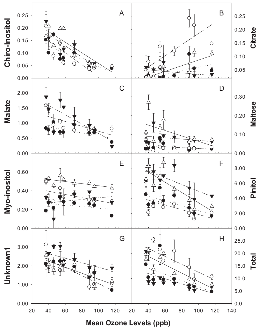
Fig. 9. Sugar profiling (unit = mmol m -2 ) analyzed with GC/MS for the young leaves (open symbol) and old leaves (closed symbol) of the 2 cultivars (DW, circle; IA, triangle) under various ozone levels at R5 stage. Linear regressions were fit for DW old (dotted line), DW young (dashed line), IA old (dot dash line) and IA young leaves (solid line), respectively. The total soluble sugars (total, H) include all of the listed in this figure plus fructose, glucose and sucrose. The overall relationships of Chiro-inositol, citrate, malate, maltose, pinitol and total with mean [O 3 ] (x) can be described as y = -0.002x + 0.241 , y = 0.0009x + 0.004 , y = -0.0126x + 2.02 , y = -0.0005x + 0.097 , y = -0.0427x + 7.42 and y = -0.1319x + 21.6 , respectively. The overall R 2 values of Chiro-inositol, citrate, malate, maltose, pinitol and total with mean [O 3 ] were significant ( p < 0.0001 ).
