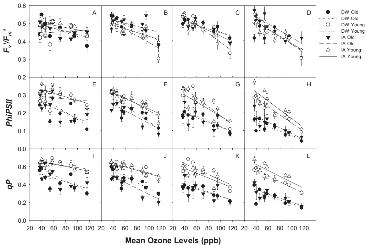
Fig. 6. F_v/F_m' (A–D), \Phi_{PSII} (E–H) and qP (I–L) for the young leaves (open symbol) and old leaves (closed symbol) of the 2 cultivars (DW, circle; IA, triangle) under various ozone levels and developmental stages – R1 (A, E and I), R2 (B, F and J), R4 (C, G and K) and R5 (D, H and L). Linear regressions were fit for DW old (dotted line), DW young (dashed line), IA old (dot dash line) and IA young leaves (solid line), respectively. The overall relationships of F_v/F_m' , \Phi_{PSII} and qP with mean [O_3] ( x ) can be described as y = -0.0013x + 0.552 , y = -0.0016x + 0.329 , and y = 0.0024x + 0.627 , respectively. The overall R^2 values of F_v/F_m' , \Phi_{PSII} and qP with mean [O_3] were significant ( p < 0.0001 ).
