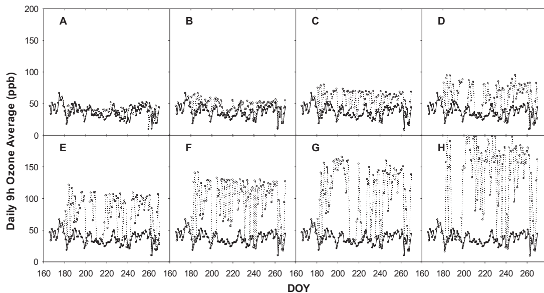
Fig. 1. Daily 9-h average ozone concentrations across the growing season for the ambient ozone concentration (closed circles, overall average 37 \pm 10 ppb) and various elevated ozone treatments (open circles). The overall average ozone concentrations for various elevated ozone treatments were 40 \pm 9 ppb (A), 46 \pm 10 ppb (B), 54 \pm 16 ppb (C), 58 \pm 21 ppb (D), 71 \pm 30 ppb (E), 89 \pm 37 ppb (F), 95 \pm 49 ppb (G) and 116 \pm 64 ppb (H).
