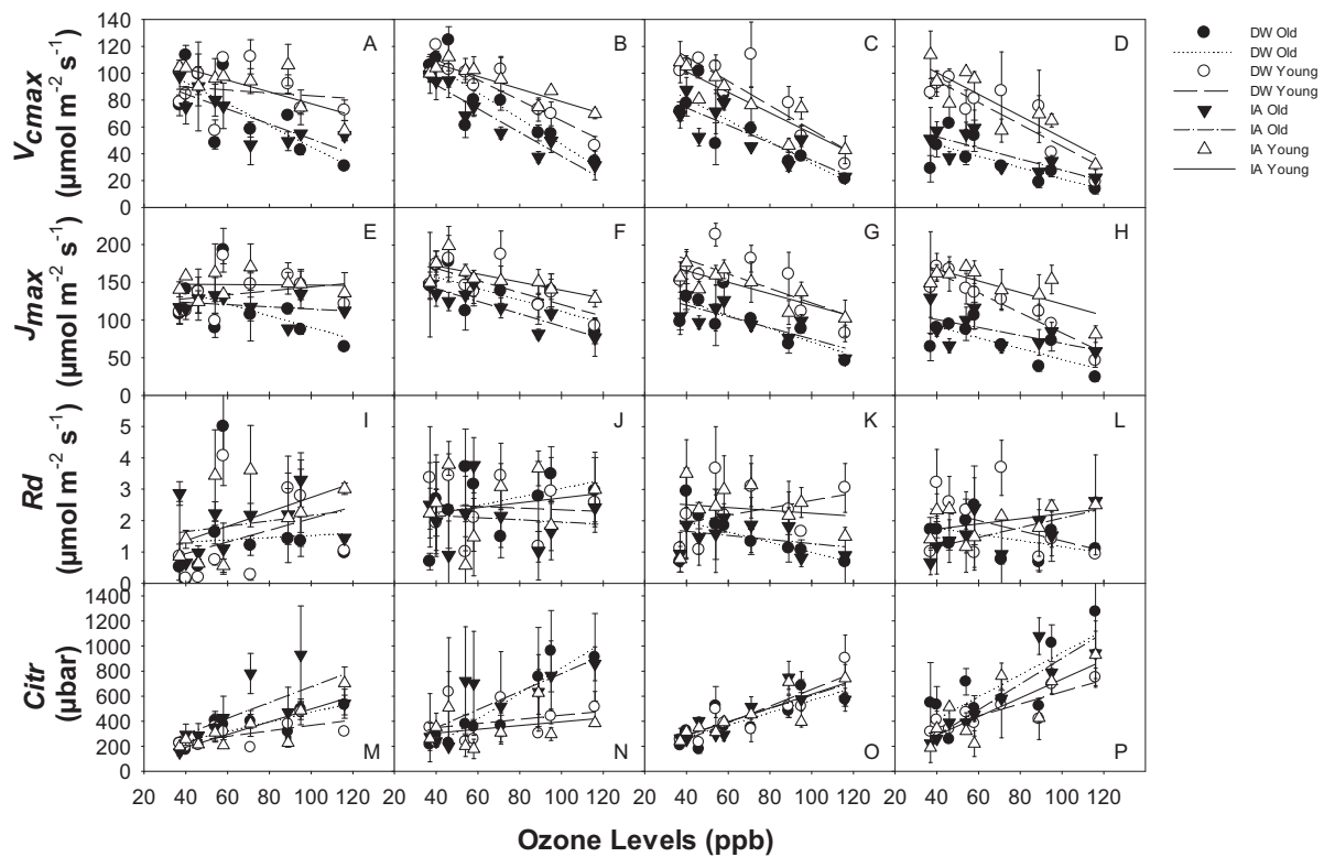
Fig. 4. V_{max} (A–D), J_{max} (E–H), R_d (I–L) and C_{itr} (M–P) for the young leaves (open symbol) and old leaves (closed symbol) of the 2 cultivars (DW, circle; IA, triangle) under various ozone levels and developmental stages – R1 (A, E, I and M), R2 (B, F, J and N), R4 (C, G, K and O) and R5 (D, H, L and P). Linear regressions were fit for DW old (dotted line), DW young (dashed line), IA old (dot dash line) and IA young leaves (solid line), respectively. The overall relationships of V_{max} , J_{max} and C_{itr} with mean [O_3] ( x ) can be described as y = -0.65x + 116 , y = -0.65x + 169 , and y = 0.41x + 267 , respectively. The overall R^2 values of V_{max} , J_{max} and C_{itr} with mean [O_3] were significant ( p < 0.0001 ).
