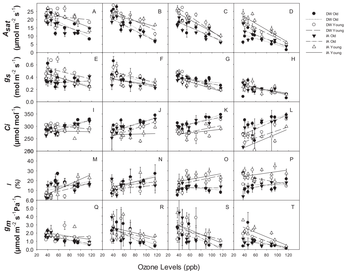
Fig. 3. A_{sat} (A–D), g_s (E–H), C_i (I–L), l (M–P) and g_m (Q–T) for the young leaves (open symbol) and old leaves (closed symbol) of the 2 cultivars (DW, circle; IA, triangle) under various ozone levels and developmental stages – R1 (A, E, I, M and Q), R2 (B, F, J, N and R), R4 (C, G, K, O and S) and R5 (D, H, L, P and T). Linear regressions were fit for DW old (dotted line), DW young (dashed line), IA old (dot dash line) and IA young leaves (solid line), respectively. The overall relationships of A_{sat} , g_s , C_i , l and g_m with mean [O_3] ( x ) can be described as y = -0.152x + 27 , y = -0.0021x + 0.4752 , y = 0.406x + 267 and y = 0.077x + 11 , and y = -0.02x + 2.86 , respectively. The overall R^2 values of A_{sat} , g_s , C_i , l and g_m with mean [O_3] were significant ( p < 0.001 ).
