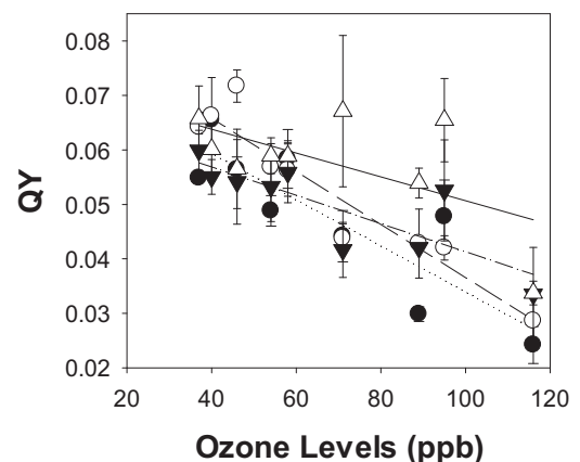
Fig. 5. QY for the young leaves (open symbol) and old leaves (closed symbol) of the 2 cultivars (DW, circle; IA, triangle) under various ozone levels at R5 stage. Linear regressions were fit for DW old (dotted line), DW young (dashed line), IA old (dot dash line) and IA young leaves (solid line), respectively. The overall relationship of QY with mean [O_3] ( x ) can be described as y = -0.003x + 0.075 . The overall R^2 between QY and mean [O_3] was significant ( p < 0.0001 ).
