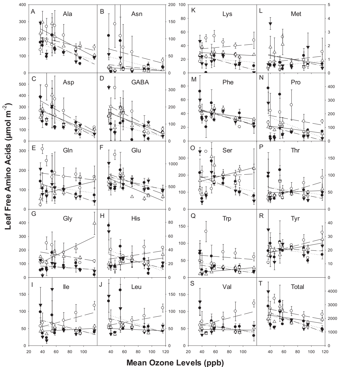
Fig. 10. Amino acids profiling (unit = \mu\text{mol m}^{-2} ) in the young leaves (open symbol) and old leaves (closed symbol) of the 2 cultivars (DW, circle; IA, triangle) under various ozone levels at R5 stage. Linear regressions were fit between ozone levels and each of the free amino acids for DW old (dotted line), DW young (dashed line), IA old (dot dash line) and IA young leaves (solid line).
